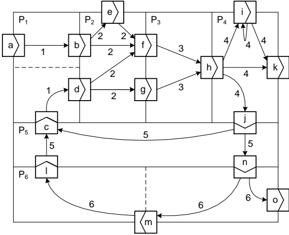
Figure 3: A passage partitioning for graph G_2 .
