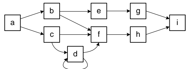
Figure 1: Graph G_1 with 9 vertices, 12 edges, and 32 passages.
