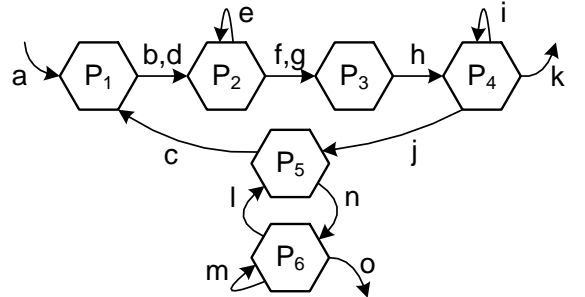
Figure 4: Passage graph based on the passage partitioning shown in Figure 3.
