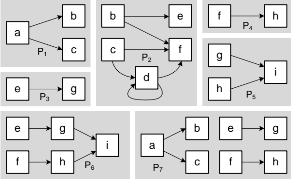
Figure 2: Seven example passages of graph G_1 shown in Figure 1.
