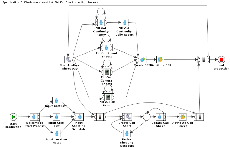
Fig. 4. Film Production Process (using YAWL [18] notation).
