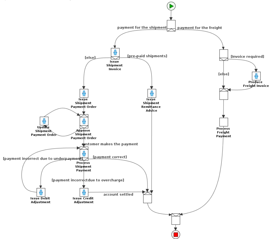
Fig. 6. Order Fulfillment Process: Payment Subprocess (using YAWL [18] notation).
