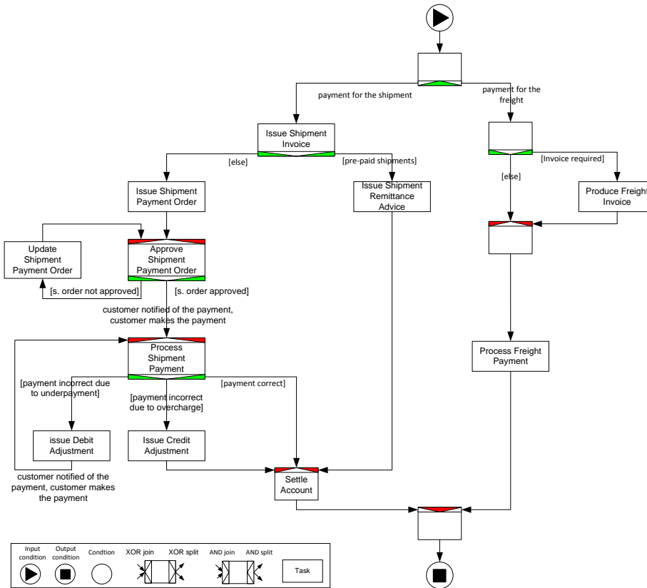
Fig. 2. Order-Fulfillment: Payment subprocess (using YAWL [18] notation).
