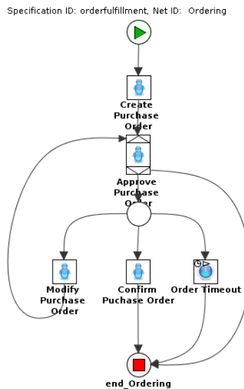
Fig. 5. Order Fulfilment Process: Ordering Subprocess (using YAWL [18] notation).
