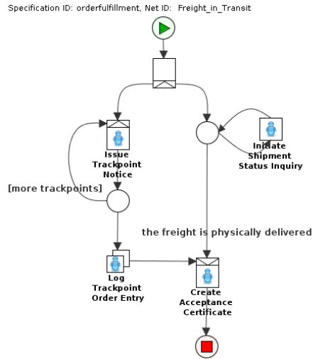
Fig. 7. Order Fulfilment Process: Freight in Transit Subprocess (using YAWL [18] notation).
