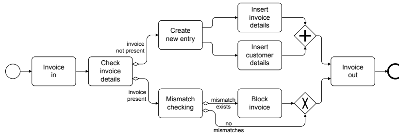
Fig. 7. Alternative Representation of splits and joins for the model in Figure 3b.
