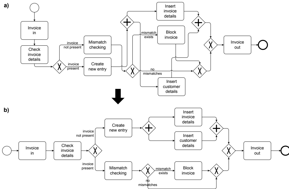
Fig. 3. a) A BPMN model not following any layout guidelines. b) The same model after applying the BPMN layout guidelines.
