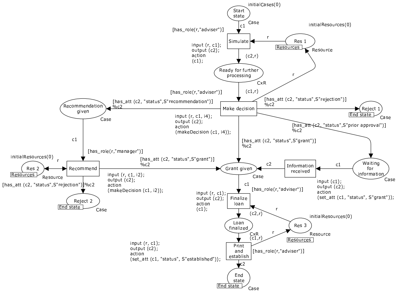
Figure 9. CWN model of a blanc loan process.
