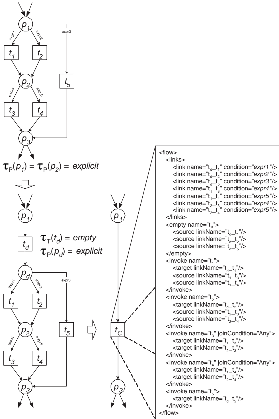
Figure 6. Example of a FLOW-component and its corresponding BPEL expression.
