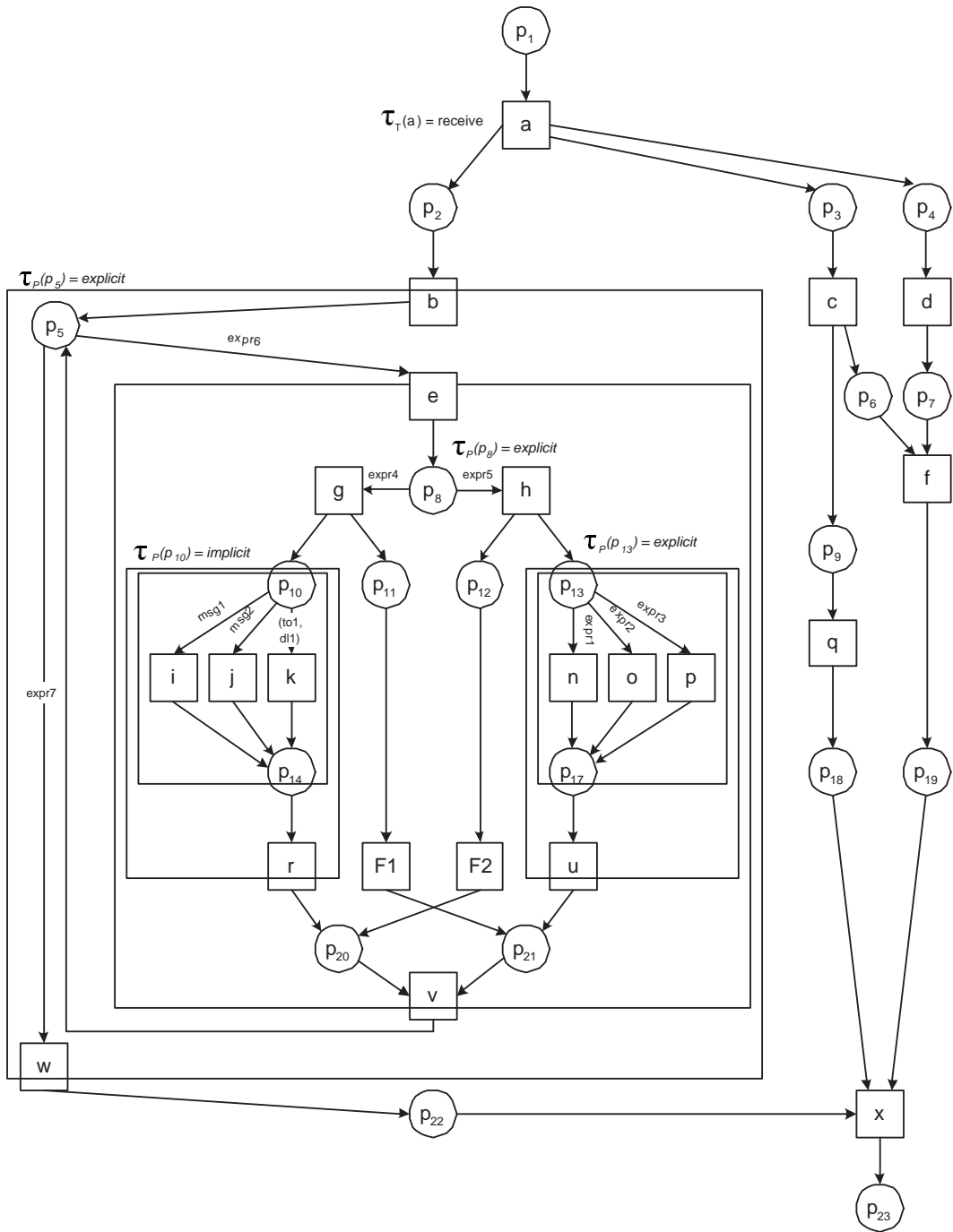
Figure 12. The WF-net after folding the two sequences.
