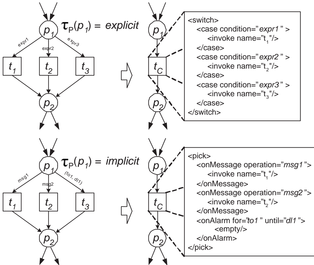
Figure 7. Examples of the SWITCH-component and PICK-component and their corresponding BPEL expression.
