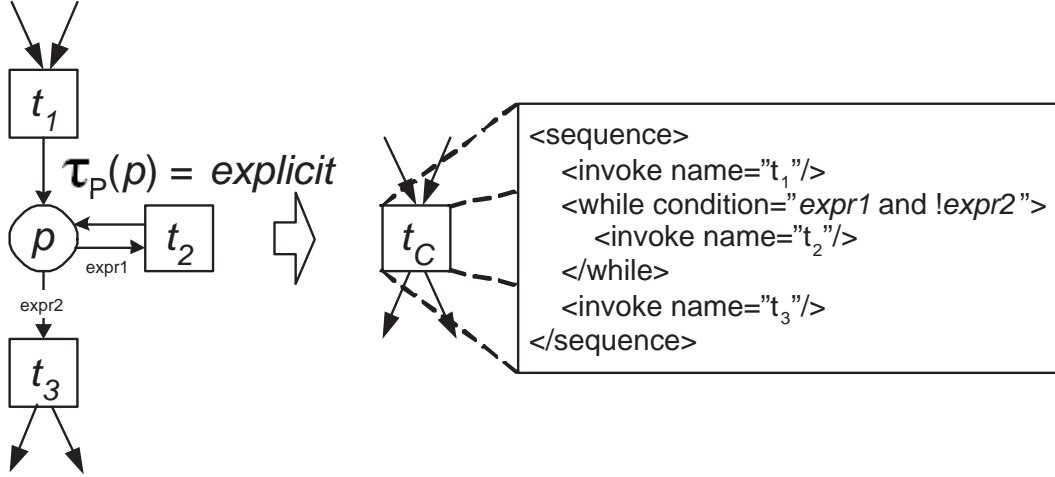
Figure 8. Example of the WHILE-component and its corresponding BPEL expression.
