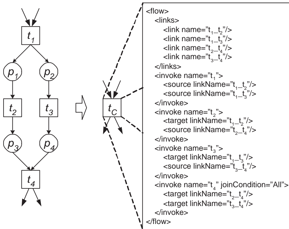
Figure 5. Examples of the FLOW-component and its corresponding BPEL expression.
