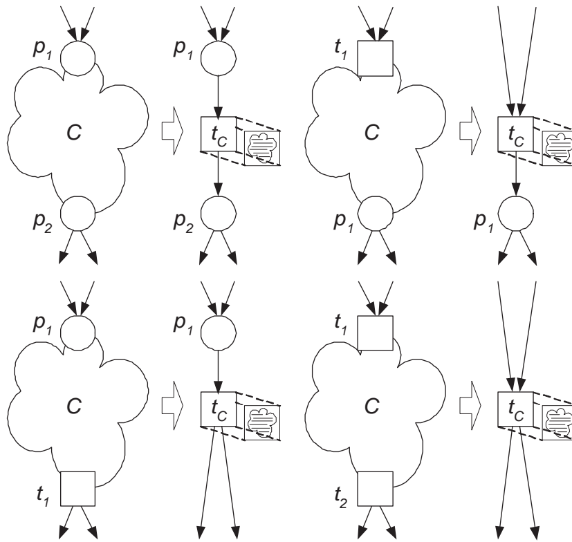
Figure 1. Folding a component C into a single transition t_C .
