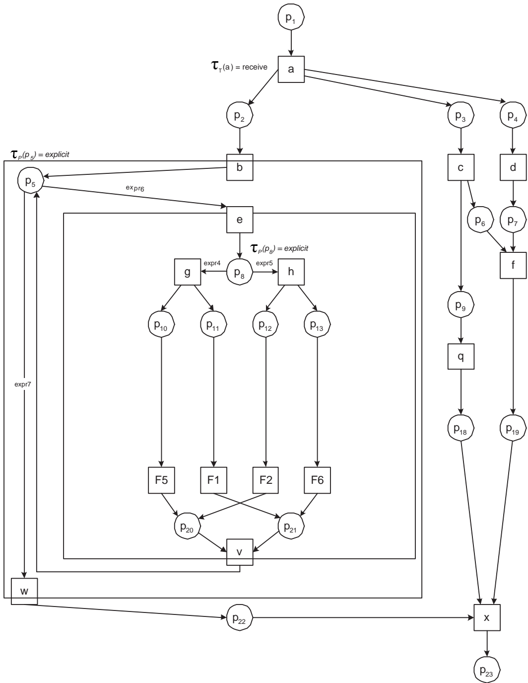
Figure 14. The WF-net after folding the two new sequences.
