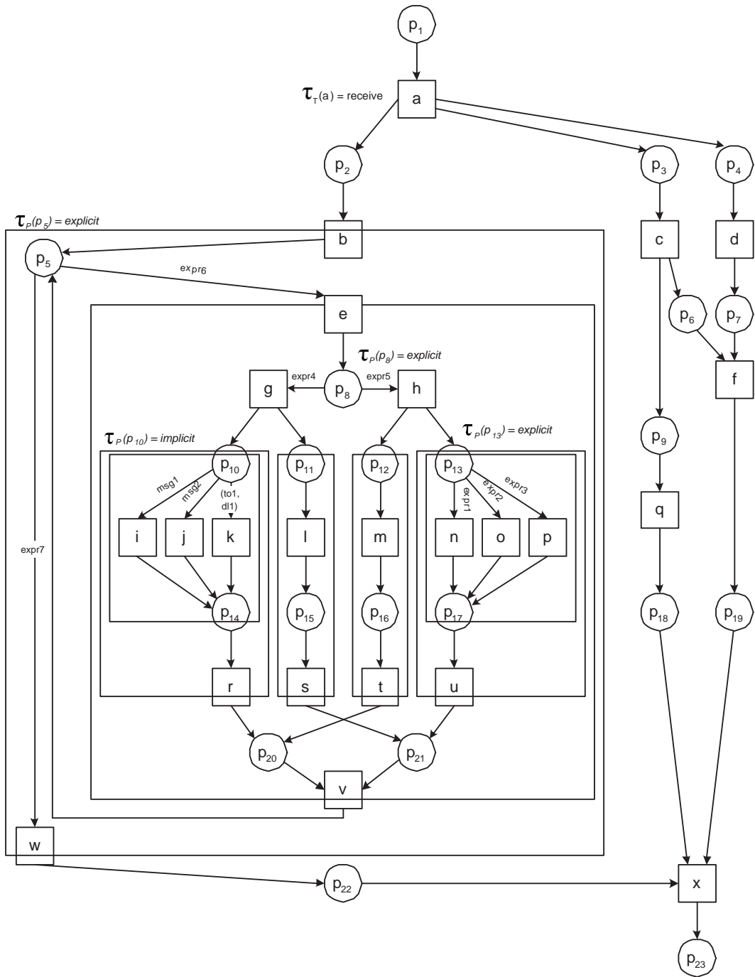
Figure 11. The original WF-net before reduction.
