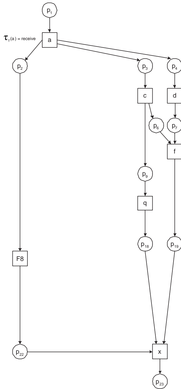
Figure 16. The WF-net after folding the while construct. The resulting WF-net is a marked graph and can be mapped onto a BPEL flow.
