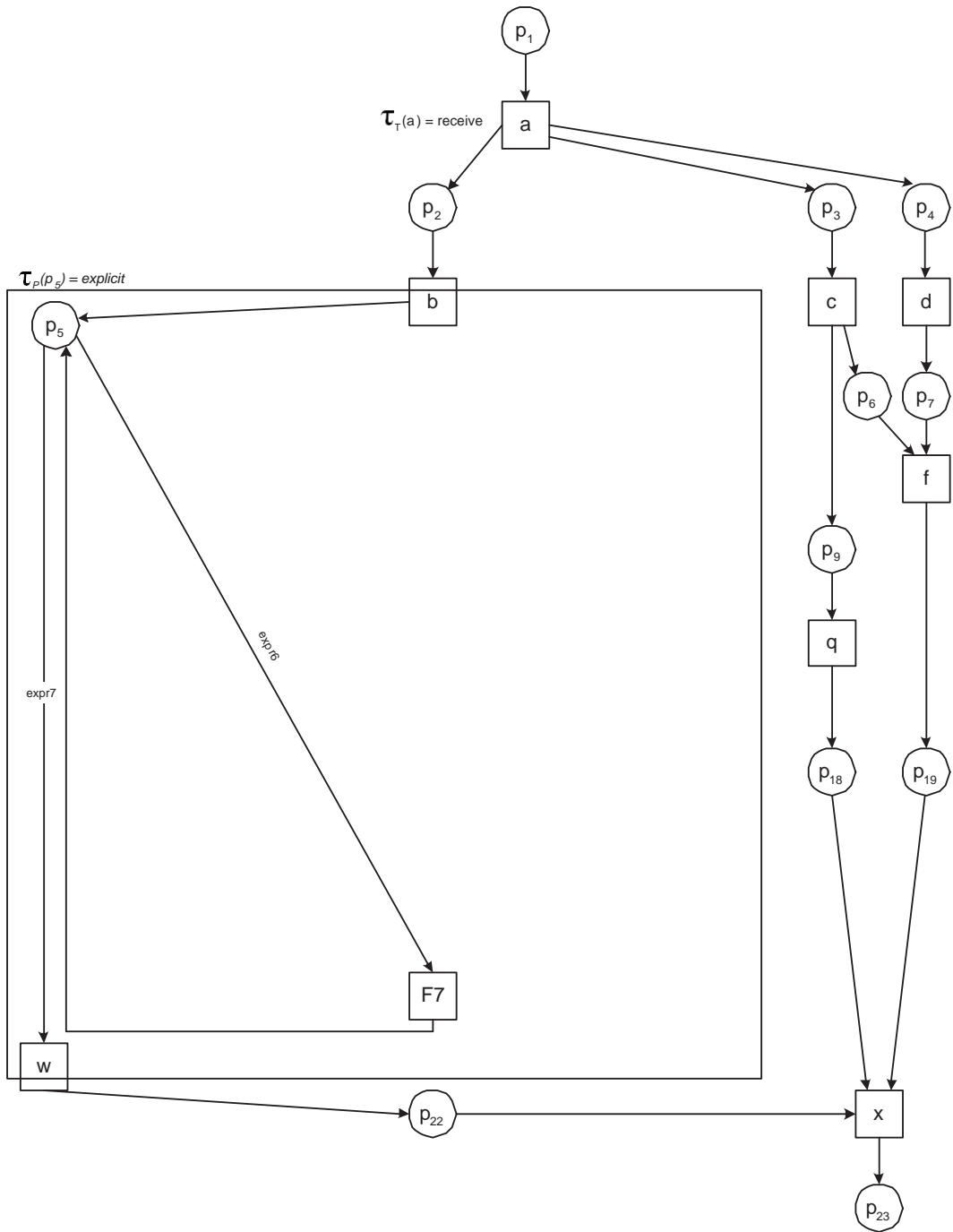
Figure 15. The WF-net after folding the ad-hoc component.
