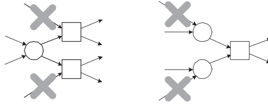
Figure 3. Two constructs not allowed in a well-structured Petri net.
