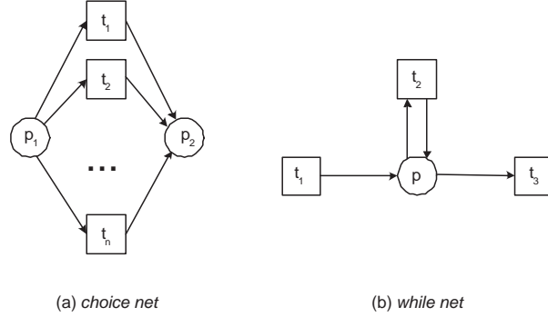
Figure 2. Two subclasses (while net and choice net) inspired by the switch , pick and while in BPEL.
