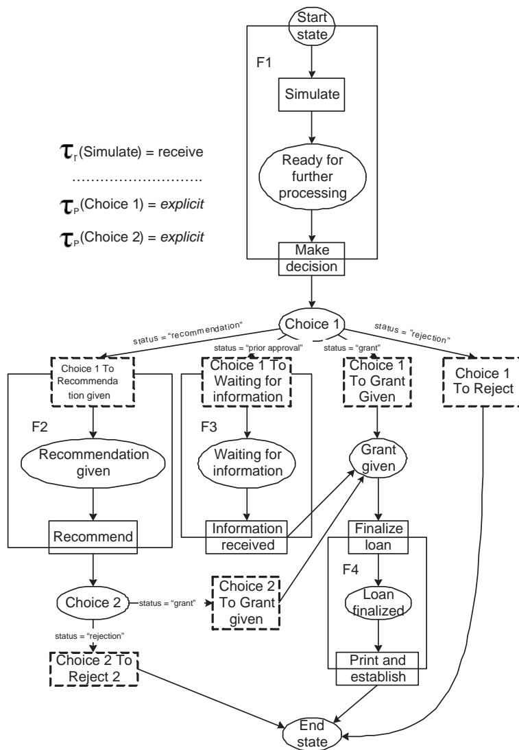
Figure 10. WF model of a blanc loan process.
