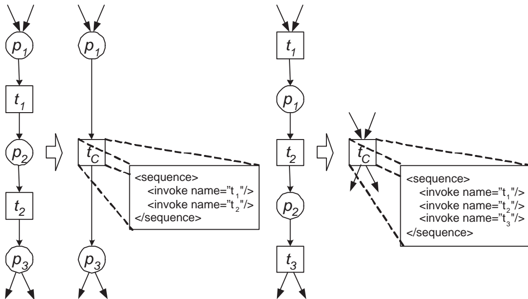
Figure 4. Examples of the SEQUENCE-component and its corresponding BPEL expression.
