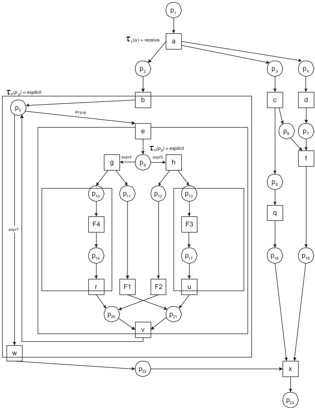
Figure 13. The WF-net after folding the switch and pick.
