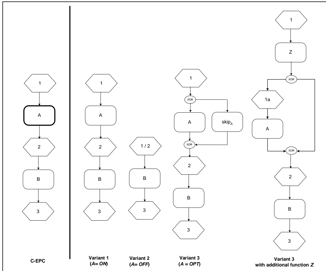
Fig. 6: Example for a configuration with additional elements
